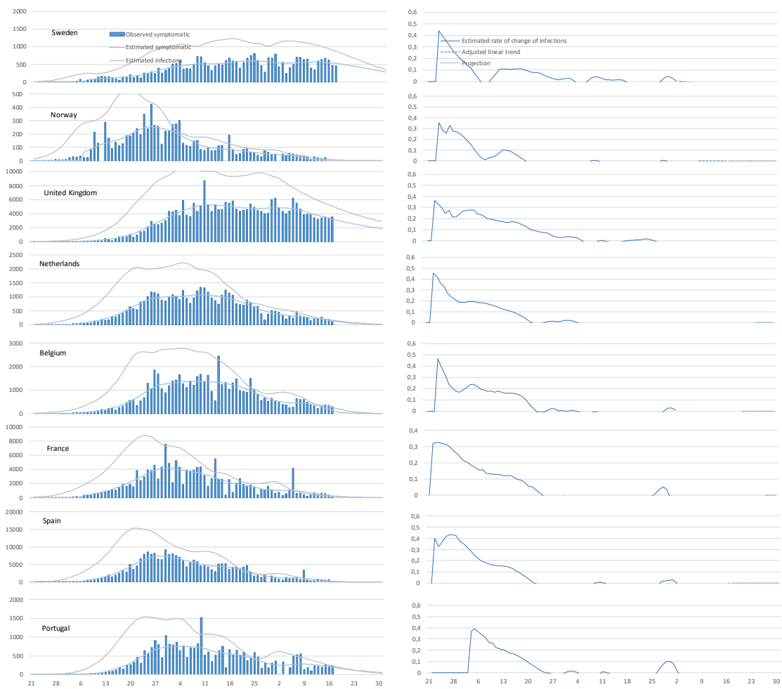
Figure 3. Observed and estimated symptomatic cases and number of infections in Western Europe.
