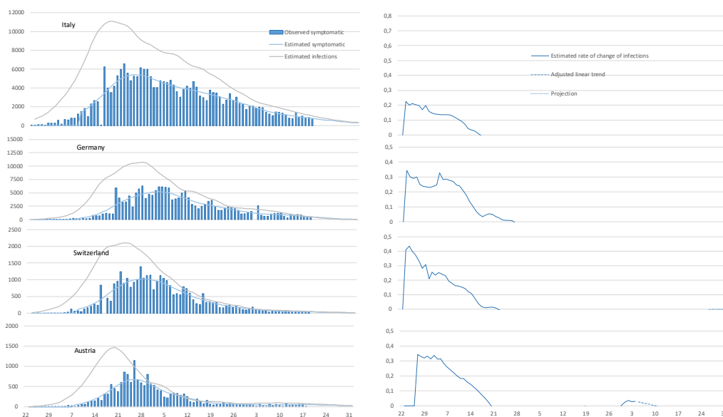
Figure 4. Observed and estimated symptomatic cases and number of infections in Italy, Switzerland, Germany and Austria, showing that the number of infections is already decreasing significantly in all countries, even if new increases are possible.
