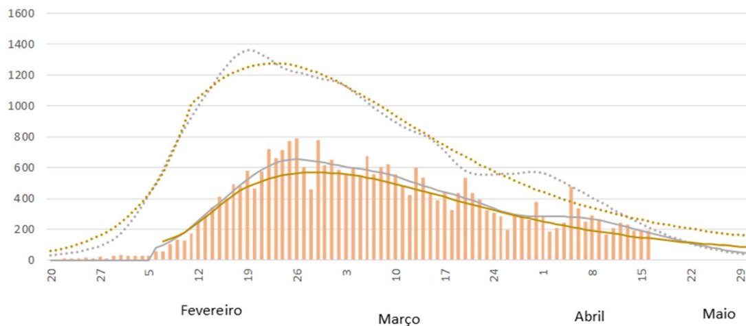
Figure 1. Analysis of the estimated dynamics of transmissions and symptomatic cases estimated by two different models for Portugal from February 20 to May 16, and the projections for the period May 17 to May 30, modelled from DGS data. The assumptions of the incubation period and the asymptomatic rates are in the model.
