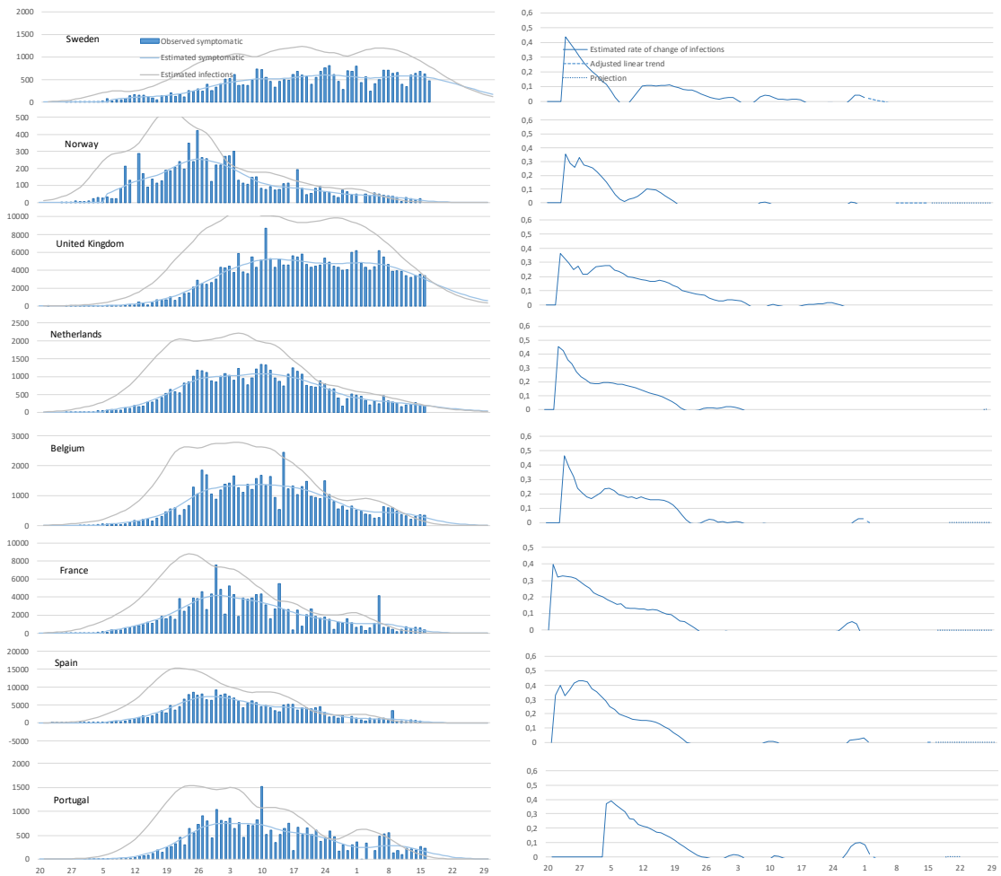
Figure 4. Observed and estimated symptomatic cases and number of infections in Western Europe.
