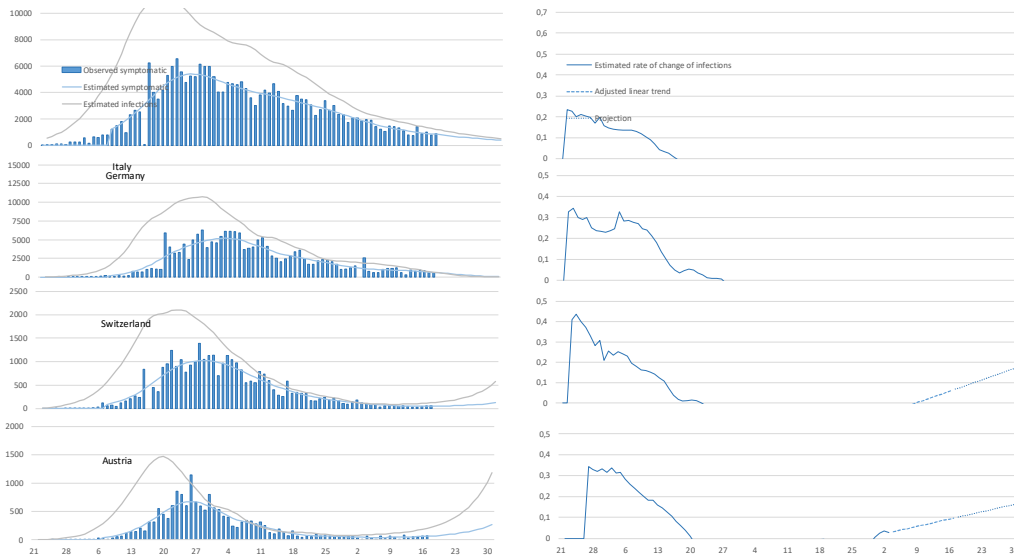
Figure 5. Observed and estimated symptomatic cases and number of infections in Italy, Switzerland, Germany and Austria, showing that the number of infections is already decreasing significantly in all countries, even if new increases are possible.
