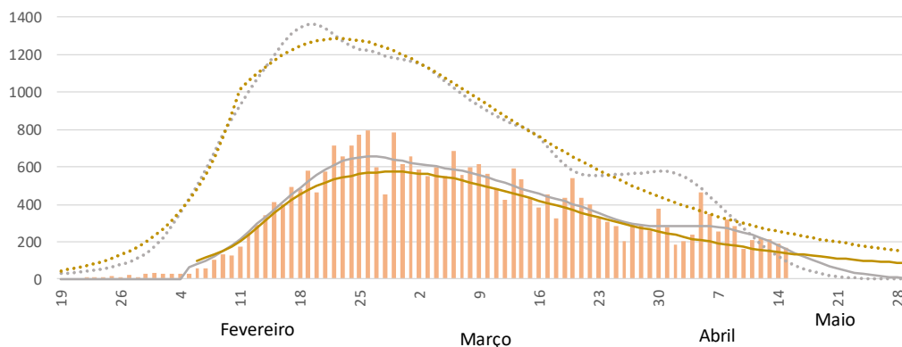
Figure 1. Analysis of the estimated dynamics of transmissions and symptomatic cases estimated by two different models for Portugal from February 19 to May 15, and the projections for the period May 16 to May 29, modelled from DGS data. The assumptions of the incubation period and the asymptomatic rates are in the model.
