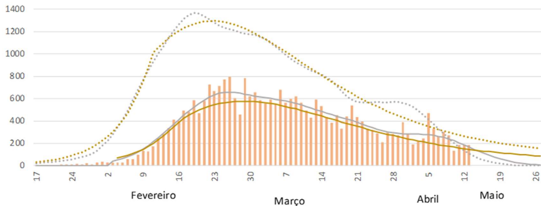
Figure 1. Analysis of the estimated dynamics of transmissions and symptomatic cases estimated by two different models for Portugal from February 17 to May 13, and the projections for the period May 14 to May 27, modelled from DGS data. The assumptions of the incubation period and the asymptomatic rates are in the model.
