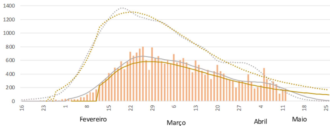
Figure 1. Analysis of the estimated dynamics of transmissions and symptomatic cases estimated by two different models for Portugal from February 16 to May 12, and the projections for the period May 13 to May 26, modelled from DGS data. The assumptions of the incubation period and the asymptomatic rates are in the model.
