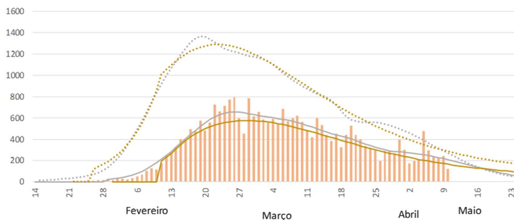
Figure 1. Analysis of the estimated dynamics of transmissions and symptomatic cases estimated by two different models for Portugal from February 14 to May 10, and the projections for the period May 11 to May 24, modelled from DGS data. The assumptions of the incubation period and the asymptomatic rates are in the model.
