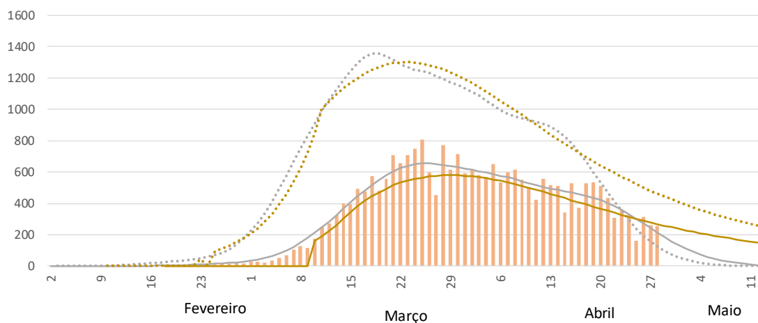
Figure 1. Analysis of the estimated dynamics of transmissions and symptomatic cases estimated by two different models for Portugal from February 3 to April 29, and the projections for the period April 30 to May 13, modelled from DGS data. The assumptions of the incubation period and the asymptomatic rates are in the model.
