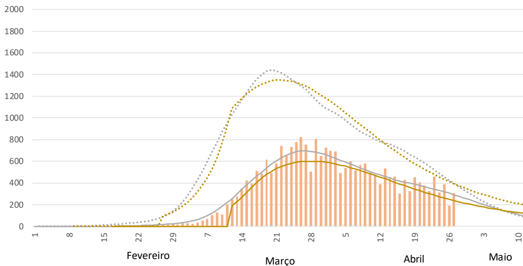
Figure 1. Analysis of the estimated dynamics of transmissions and symptomatic cases estimated by two different models for Portugal from February 1 to April 27, and the projections for the period April 28 to May 11, modelled from DGS data. The assumptions of the incubation period and the asymptomatic rates are in the model.
