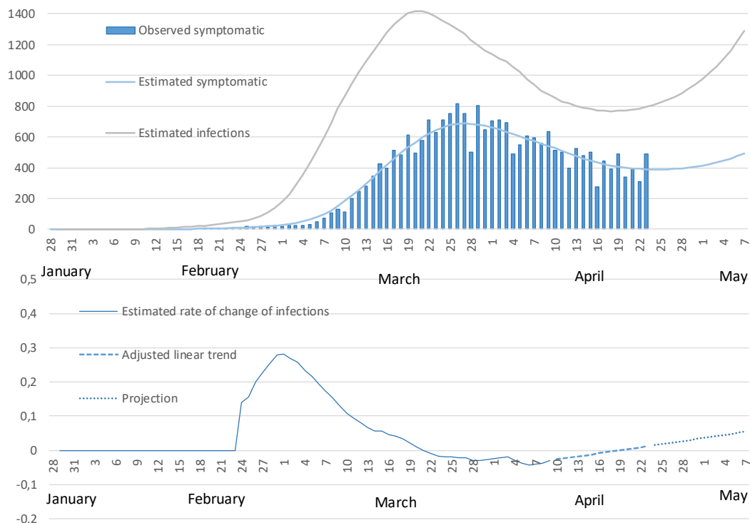
Figure 1. Analysis of the estimated dynamics of transmissions and symptomatic cases (graph at the top) and the estimated rate of change of infections (graph at the bottom) for Portugal from January 28 to April 23, and the projections for the period April 24 to May 7, modelled from DGS data. The assumptions of the incubation period and the asymptomatic rates are in the model.
