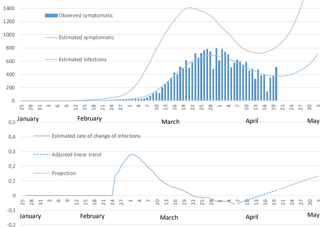
Figure 1. Analysis of the estimated dynamics of transmissions and symptomatic cases (graph at the top) and the estimated rate of change of infections (graph at the bottom) for Portugal from January 24 to April 19, and the projections for the period April 20 to May 3, modelled from DGS data. The assumptions of the incubation period and the asymptomatic rates are in the model.
