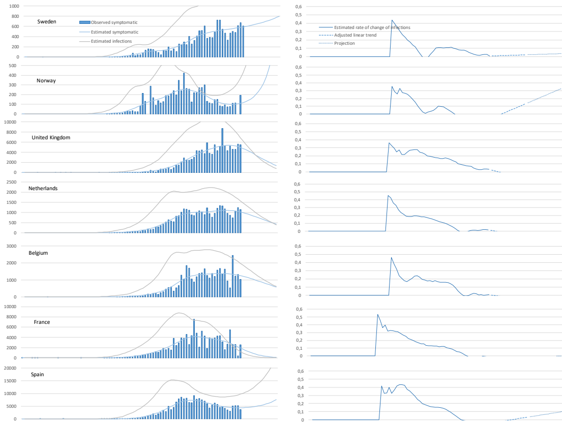
Figure 4. Observed and estimated symptomatic cases and number of infections in Sweden, Norway, United Kingdom, Netherlands, Belgium, France, and Spain.
