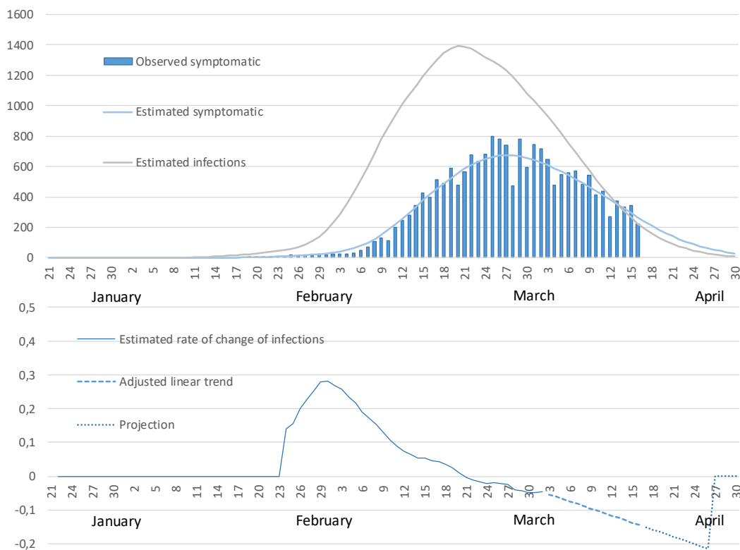
Figure 1. Analysis of the estimated dynamics of transmissions and symptomatic cases (graph at the top) and the estimated rate of change of infections (graph at the bottom) for Portugal from January 21 to April 16, and the projections for the period April 17 to April 30 modelled from DGS data. The assumptions of the incubation period and the asymptomatic rates are in the model.
