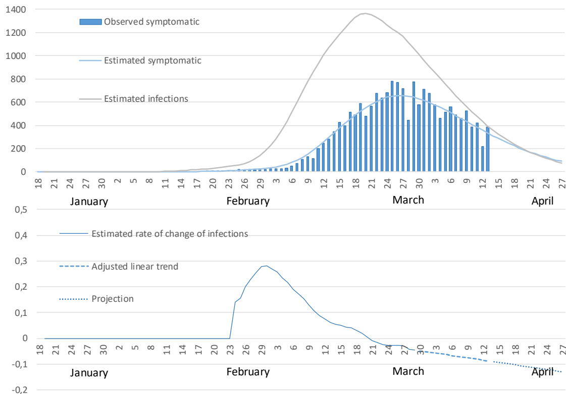
Figure 1. Analysis of the estimated dynamics of transmissions and symptomatic cases (graph at the top) and the estimated rate of change of infections (graph at the bottom) for Portugal from January 18 to April 13, and the projections for the period April 14 to April 27 modelled from DGS data. The assumptions of the incubation period and the asymptomatic rates are in the model.
