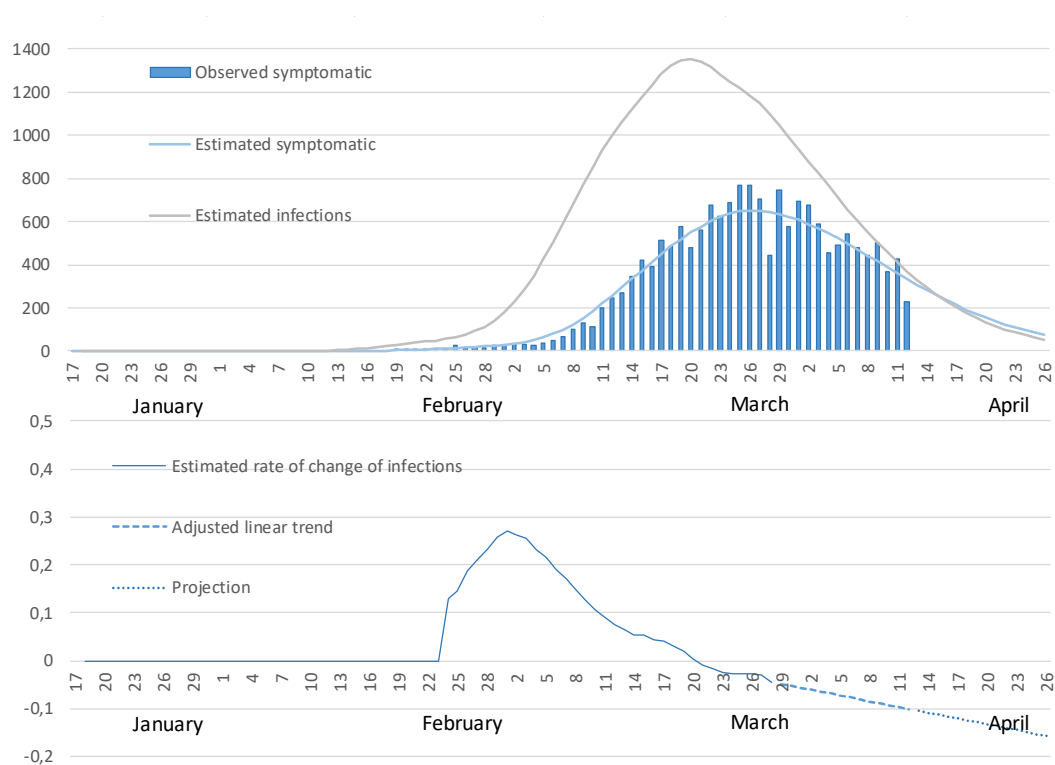
Figure 1. Analysis of the estimated dynamics of transmissions and symptomatic cases (graph at the top) and the estimated rate of change of infections (graph at the bottom) for Portugal from January 17 to April 12, and the projections for the period April 13 to April 26 modelled from DGS data. The assumptions of the incubation period and the asymptomatic rates are in the model.
